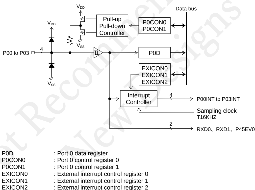
Figure 15-1 Configuration of Port 0
