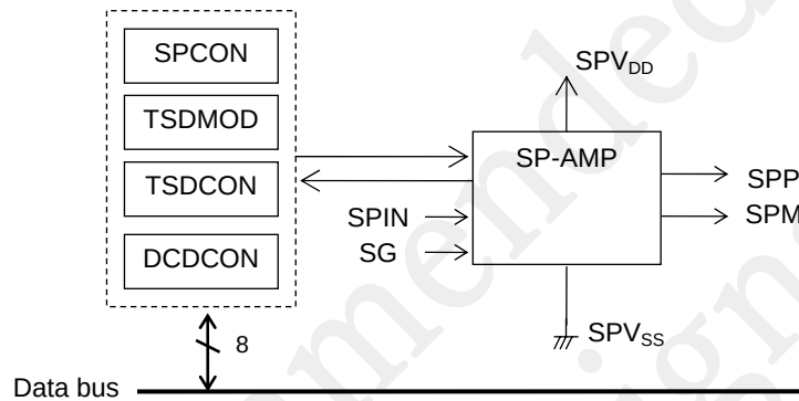
Figure 26-1 Speaker Amplifier Configuration
