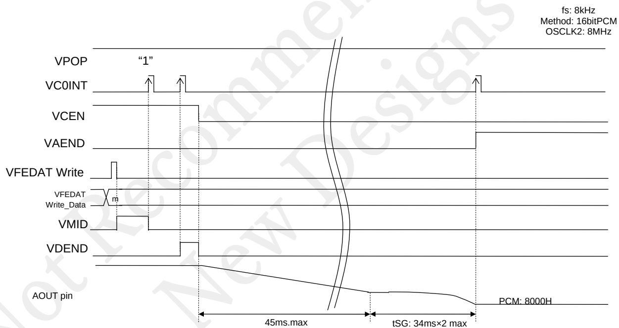
Figure 25-10 Timing Diagram of Power-down in LINE Output Mode with Pop Noise Suppression
