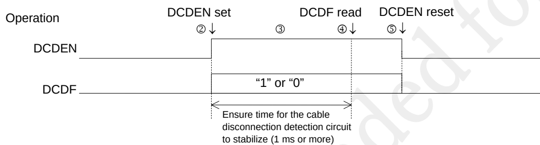
Figure 26-5 Example of Operation Timing
