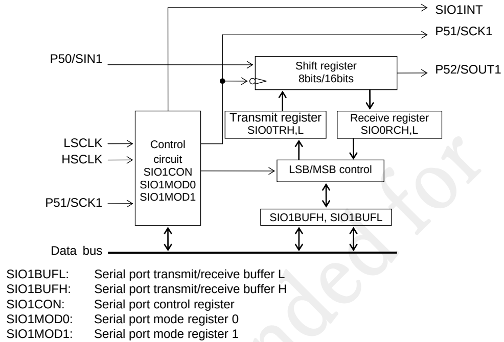
Figure 11-1 Configuration of Synchronous Serial Port
