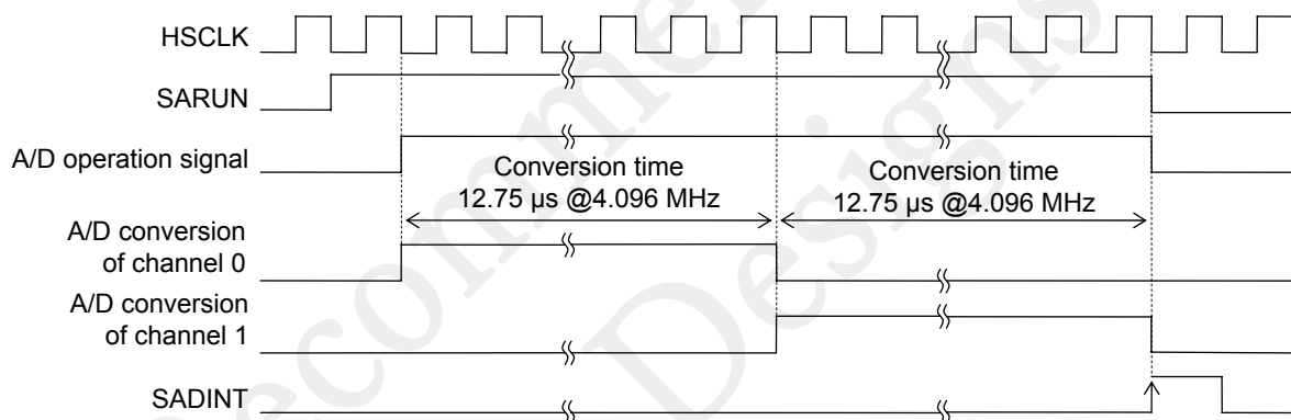
Figure 24-3 SA-ADC Operation Timing
