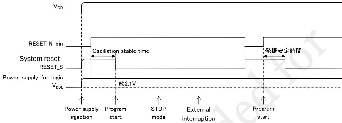
Figure 28-2 Waveforms of Power Supply Circuit Operation
