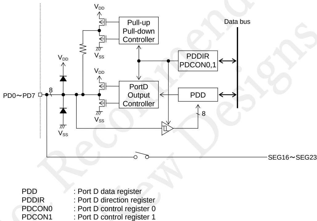
Figure 22-1 Configuration of Port D
