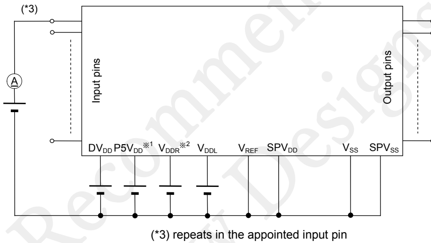
Measuring Circuit 4
