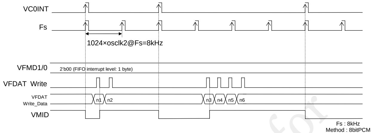
Figure 25-4 Basic Operation Timing Diagram of Audio Playback
