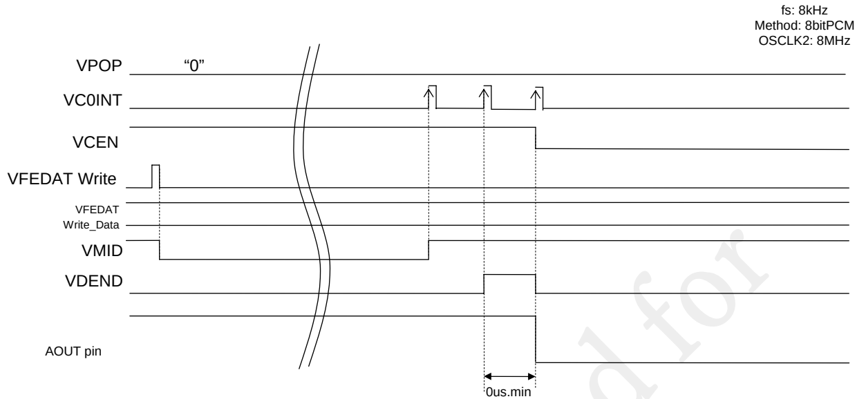
Figure 25-9 Timing Diagram of Power-down in LINE Output Mode without Pop Noise Suppression
