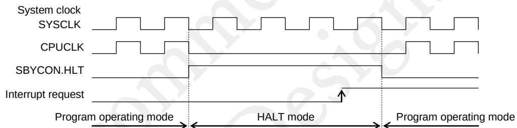
Figure 4-2 Operation Waveforms in HALT Mode
