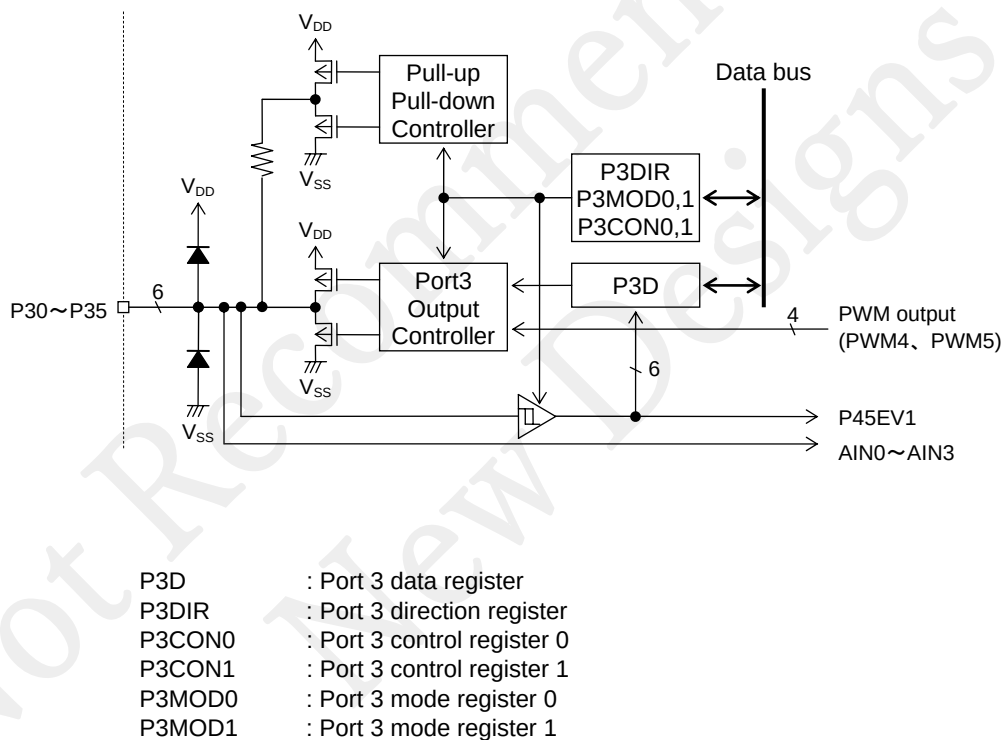
Figure 18-1 Configuration of Port 3
