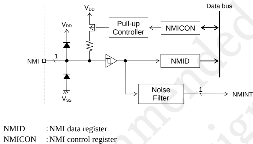
Figure 14-1 Configuration of NMI Pin
