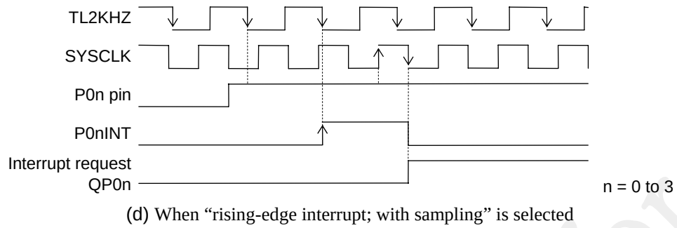
Figure 15-2 P00 to P03 Interrupt Generation Timing
