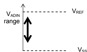
Figure 24-2 The A/D conversion pins and the conversion range
