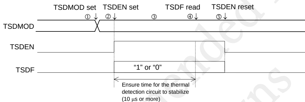
Figure 26-4 Example of Operation Timing
