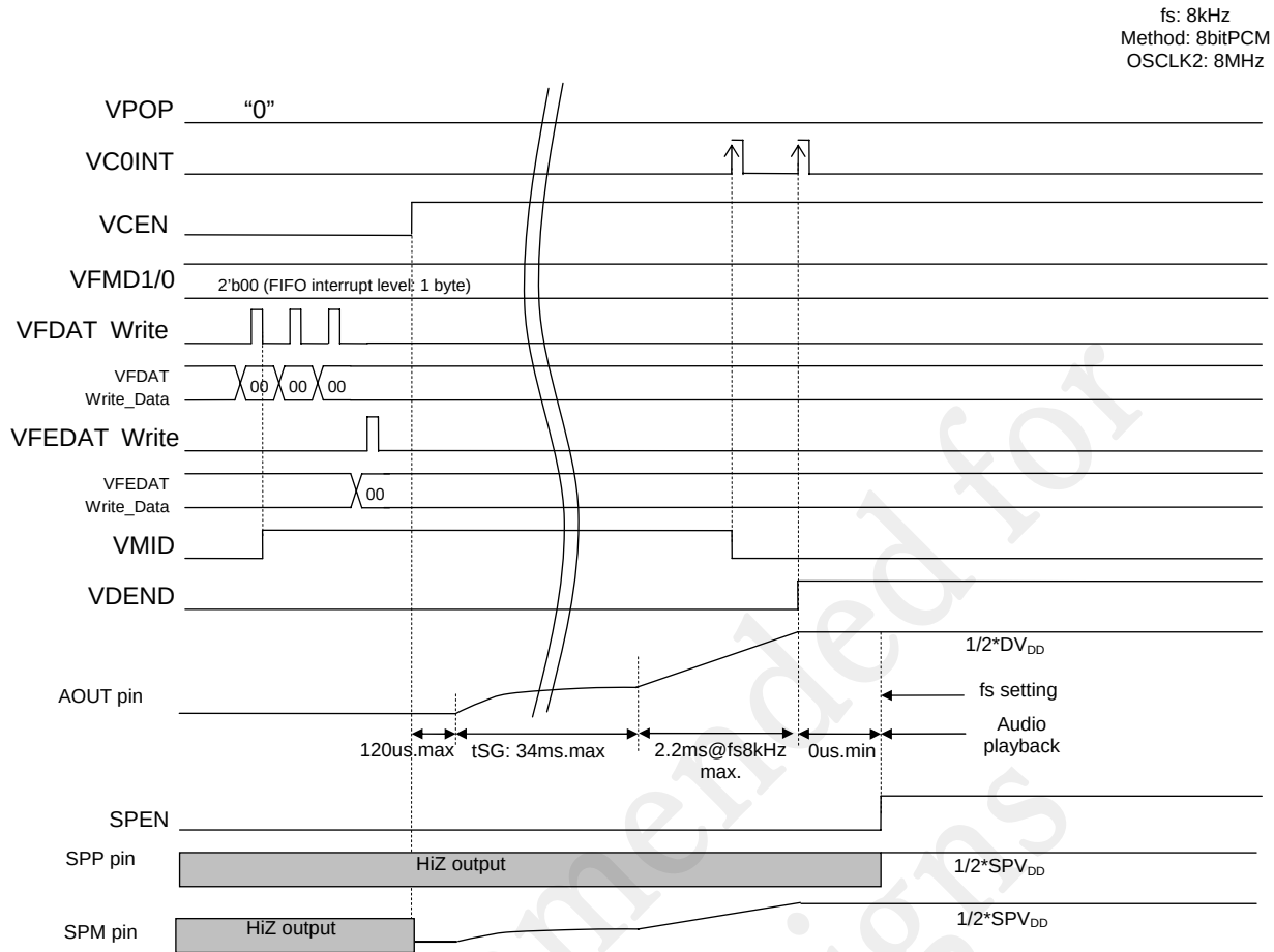
Figure 25-8 Timing Diagram of Power-up in Speaker Output Mode
