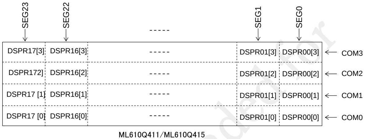
Figure 23-5 Configurations of Display register segment map
