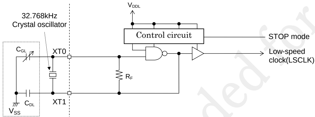
Figure 6-3 Circuit Configuration of 32.768 kHz Crystal Oscillation Mode
