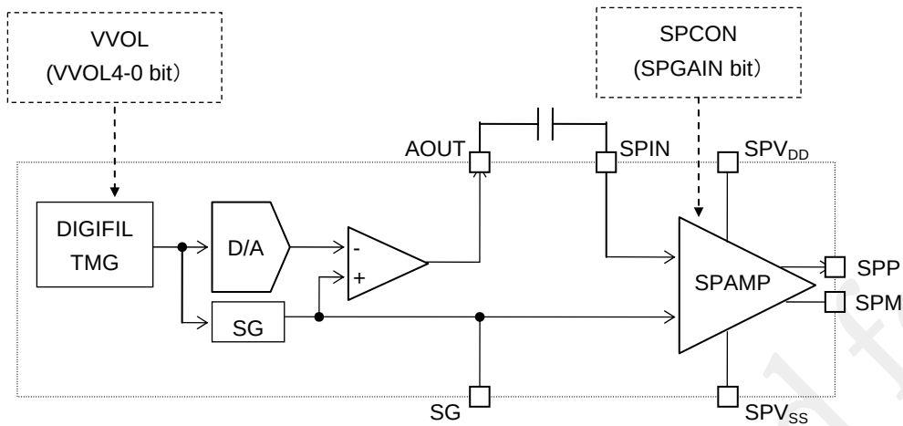
Figure 26-3 configuration relevant to volume
