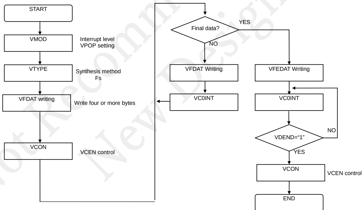
Figure 25-2 Flow Chart of Audio Playback
