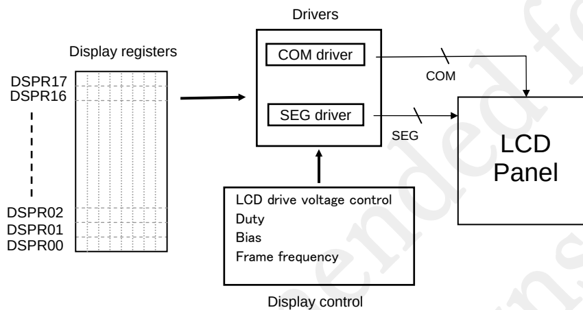
Figure 23-1 Configuration of LCD Display Function
