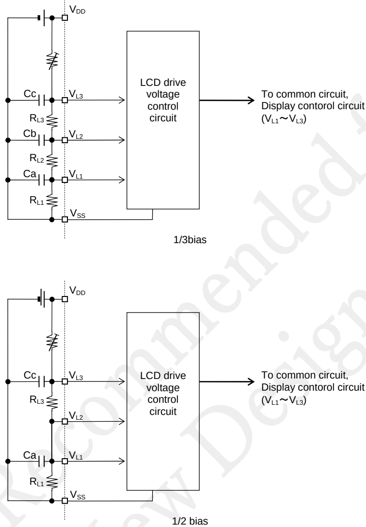
23-3 Configuration of the LCD drive voltage control circuit
