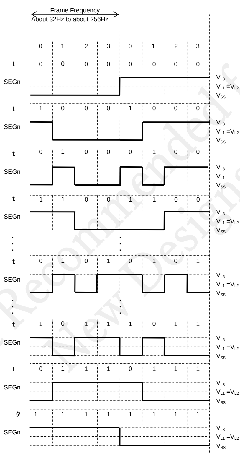
Figure 23-9 Segment Output Waveforms for 1/4 Duty and 1/2 Bias
