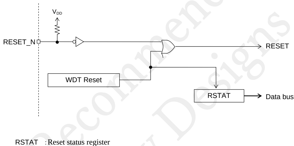
Figure 3-1 Configuration of Reset Generation Circuit
