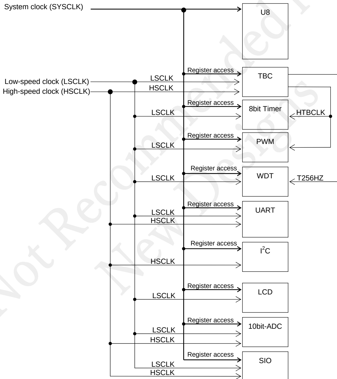
Figure 6-2 Clock Configuration
