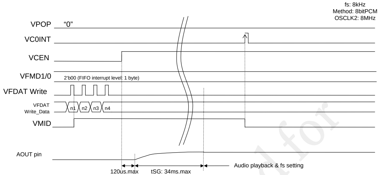
Figure 25-6 Timing Diagram of Power-up in LINE Output Mode without Pop Noise Suppression
