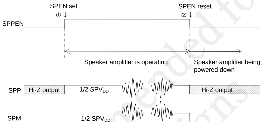
Figure 26-2 Example of Operation Timing
