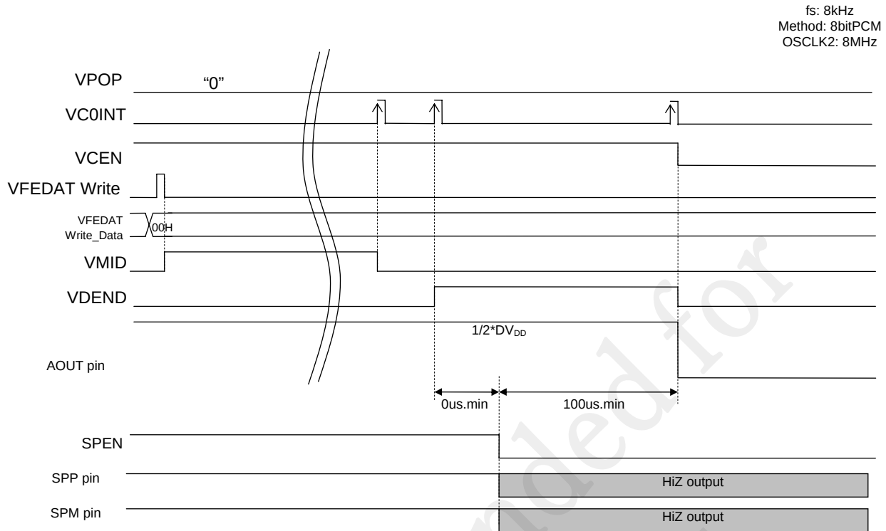
Figure 25-11 Timing Diagram of Power-down in Speaker Output Mode
