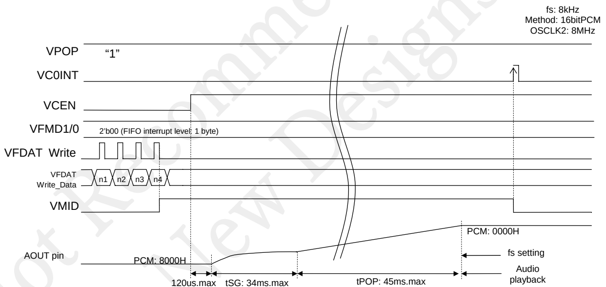
Figure 25-7 Timing Diagram of Power-up in LINE Output Mode with Pop Noise Suppression
