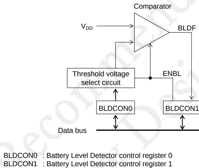
Figure 27-1 Configuration of Battery Level Detector
