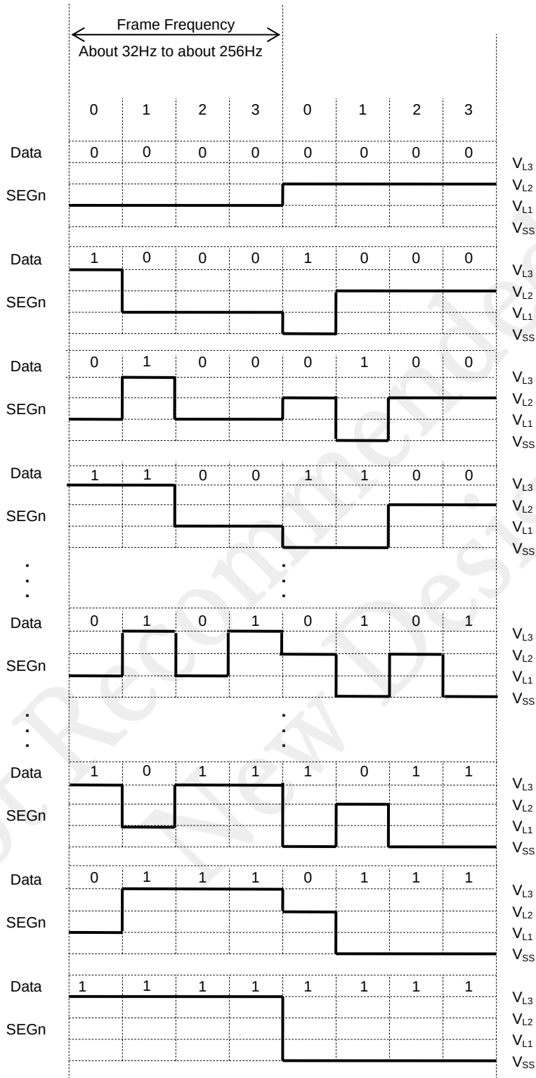
Figure 23-7 Segment Output Waveforms for 1/4 Duty and 1/3 Bias
