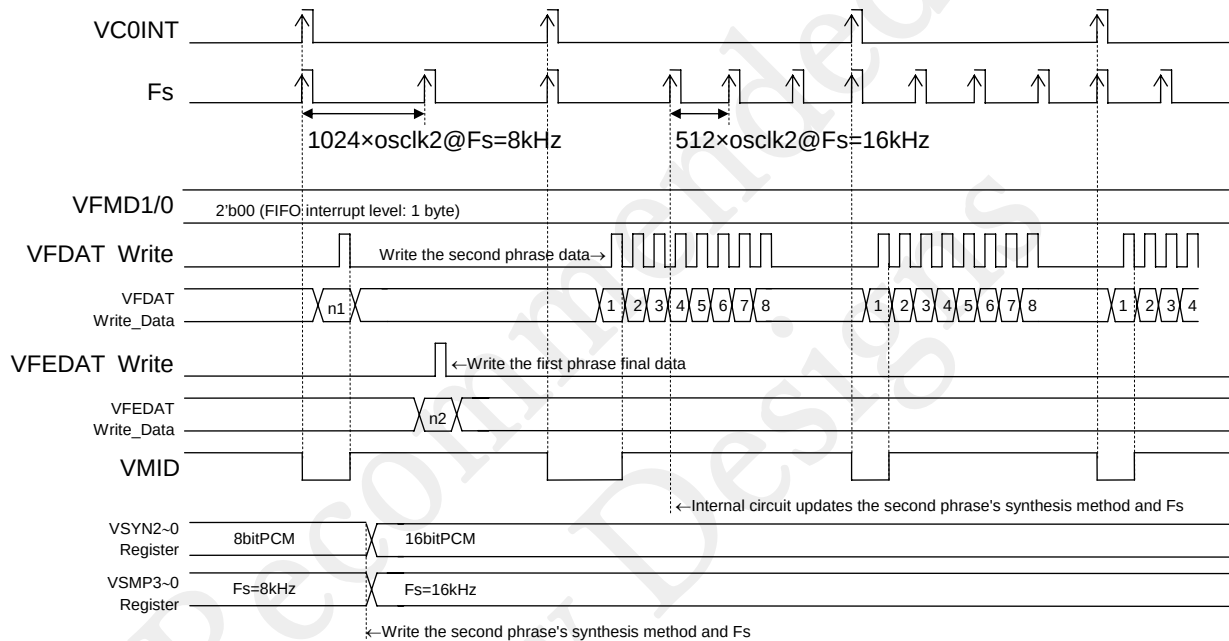
Figure 25-5 Operation Timing Diagram of Continuous Playback
