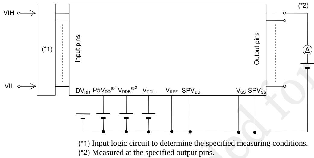
Measuring Circuit 4
