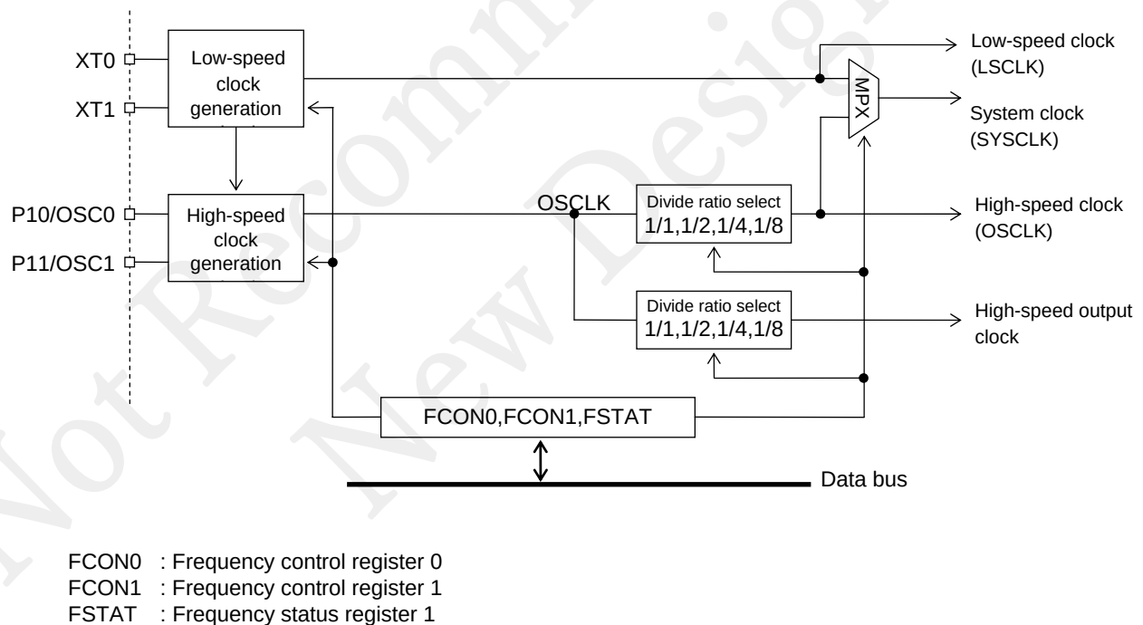
Figure 6-1 Configuration of Clock Generation Circuit
